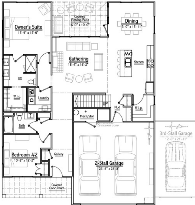
MAIN FLOOR PLAN 1,666 SQUARE FEET TOTAL SQUARE FEET TOTAL
