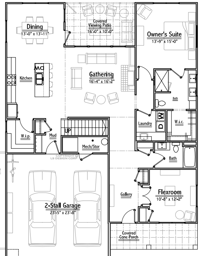
MAIN FLOOR PLAN 1,666 SQUARE FEET 1,901 SQUARE FEET TOTAL ©LS DESIGN CORP
