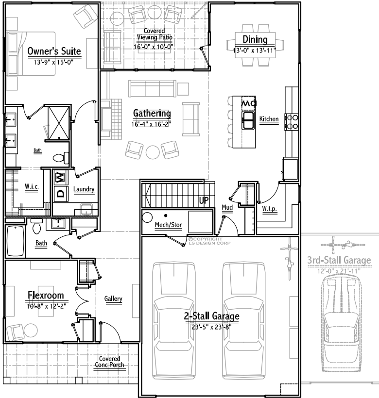
MAIN FLOOR PLAN 1,666 SQUARE FEET 1,901 SQUARE FEET TOTAL ©LS DESIGN CORP
