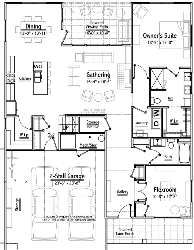
MAIN FLOOR PLAN 1,666 SQUARE FEET 1,962 SQUARE FEET TOTAL L.S. DESIGN CORP. ©
