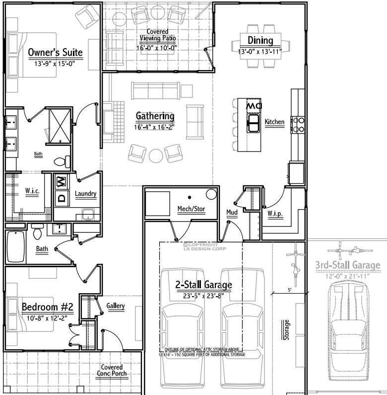
MAIN FLOOR PLAN 1,625 SQUARE FEET LS DESIGN CORP ©
